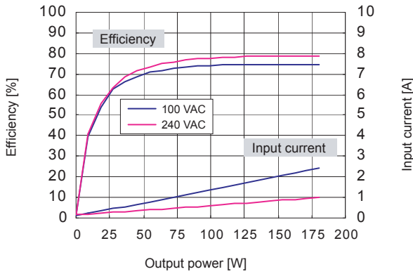
● Fig.20 Efficiency / Input Current vs. Output Power
