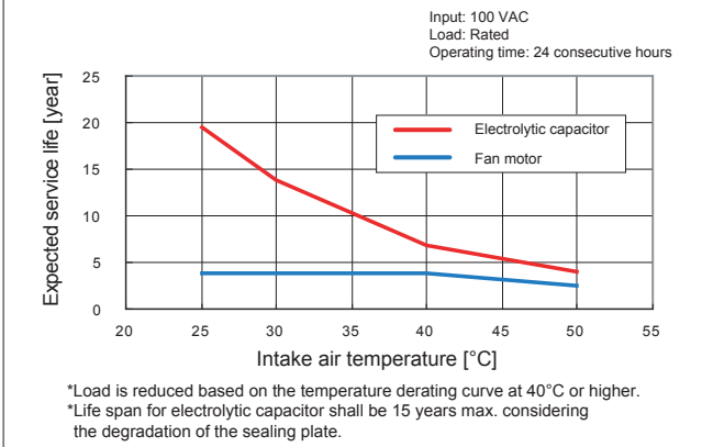
● Fig.34 Ambient Temperature vs. Expected Service Life
