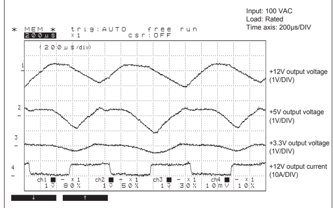
● Fig.31 Dynamic Load Fluctuation Characteristics at 1kHz
