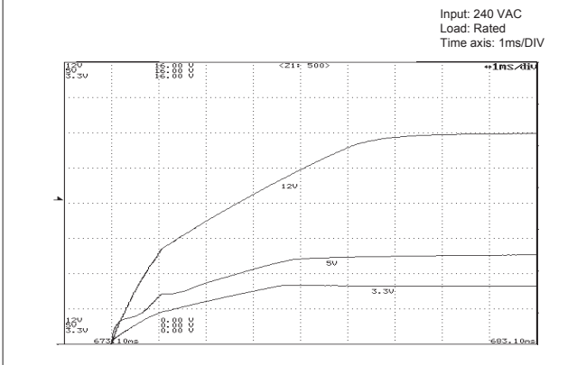
● Fig.28 Rising Characteristics at 240 VAC
