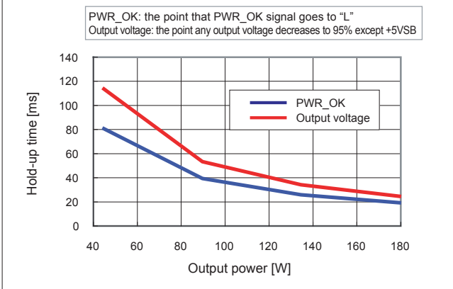
● Fig.30 Output Hold-up Time vs. Output Power
