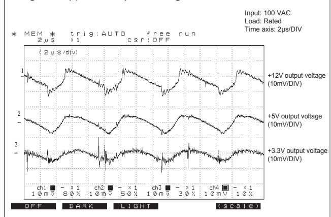
● Fig.33 Ripple and Spike Voltage
