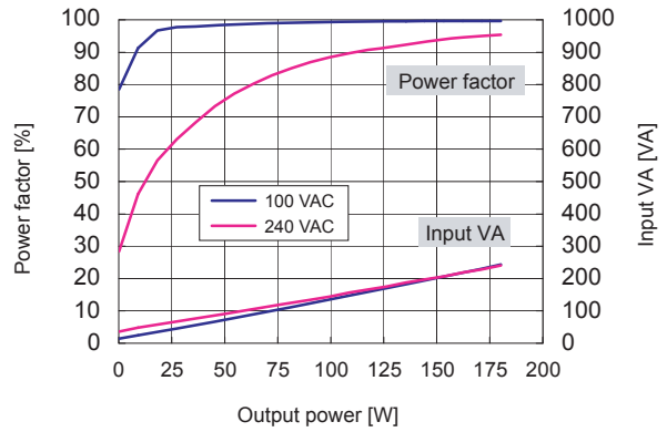
● Fig.21 Power Factor / Input VA vs. Output Power
