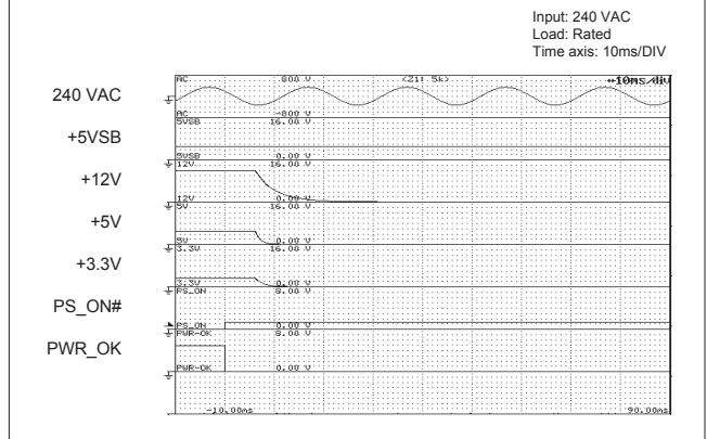
● Fig.29 Falling Characteristics at 240 VAC when REMOTE goes Off
