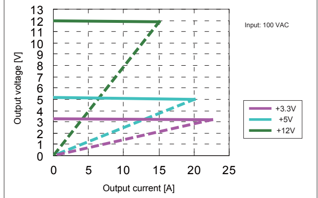
● Fig.35 Over Current Protection (V-I Characteristic)
