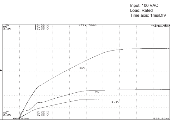
● Fig.26 Rising Characteristics at 100 VAC
